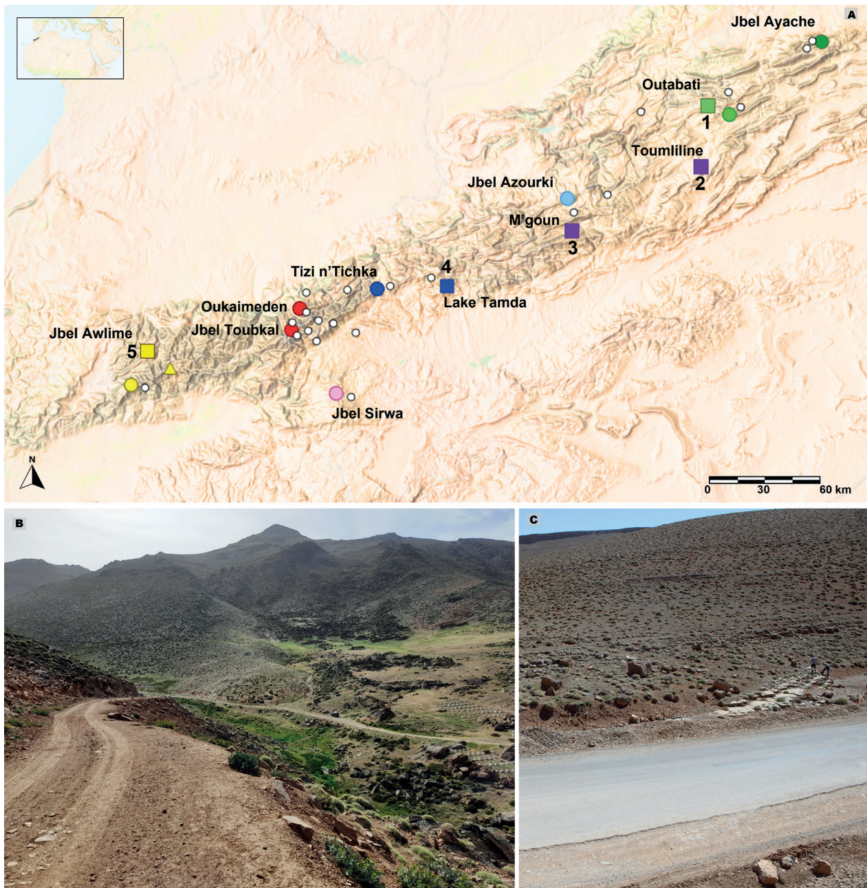
Figure 1. A. Distribution map of Atlantolacerta andreanskyi . Coloured dots are based on the distribution map populations of Barata et al. (2012). White dots represent the distribution points of Bons and Geniez (1996). The yellow triangle represents a specimen sampled in the Tichka plateau (Avella et al. 2019). The localities with newly sampled individuals are identified with numbers (1–5): Outabati (1), Toumliline (2), M'goun (3), Lake Tamda (4) and Jbel Awlime (5); B, C. Typical habitat of Atlantolacerta andreanskyi in Jbel Awlime and in Toumliline, respectively.
